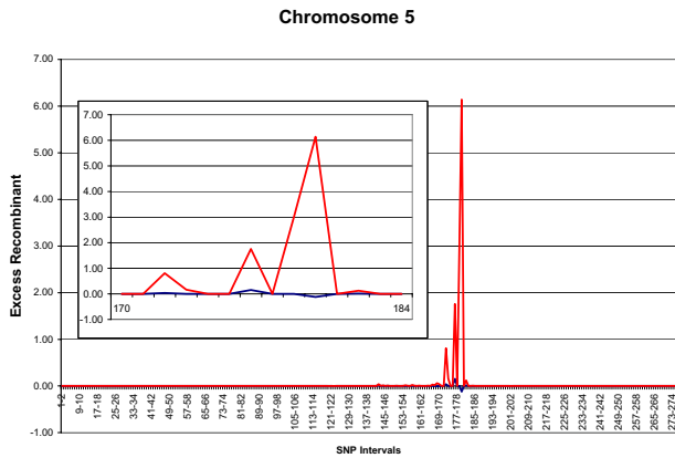
Figure 1 Distribution of excess recombinants. The red curve uses the Affymetrix genotype (tsc0260848) at marker 180. The blue curve uses the Illumina genotype (rs958883) at marker 180. The inset shows an enlarged view of the excess number of inferred recombinants in the neighborhood of rs958883/tsc0260848.
